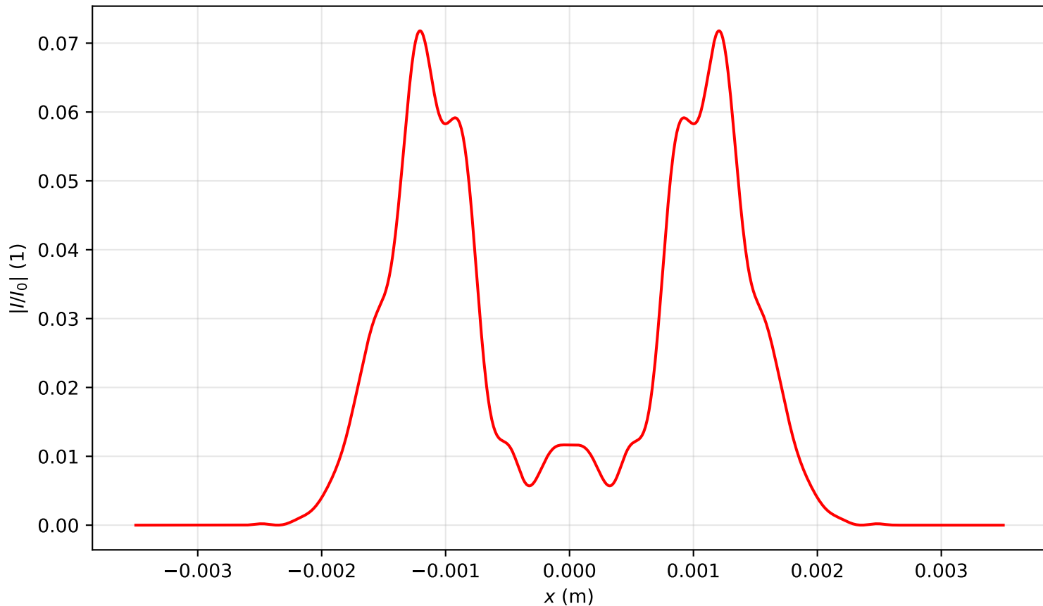
Intensity profile I(x, y = 0, z = 3.344)/I_0 , P_{in}=6.5P_{cr} , artificial time
